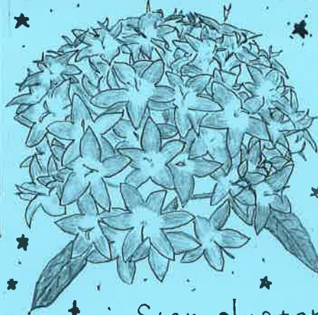
Star cluster
